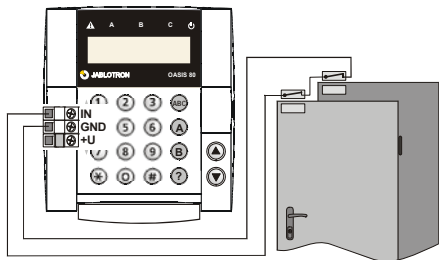
An example of door detector wiring.
